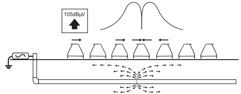
(Note that the A-frame is not shown connected to the receiver so as to simplify the diagram)
