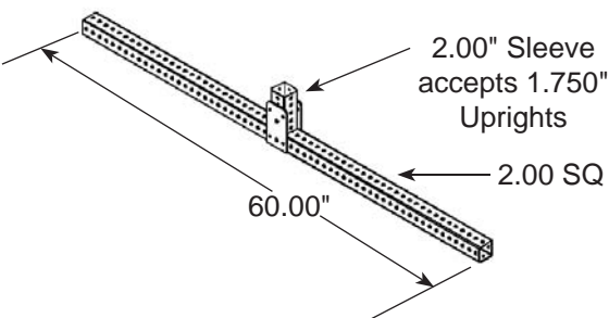
PSST Breakaway Base 14 gauge weight: 13.2 lbs.
