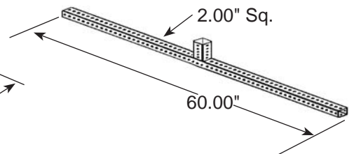
PSST Base with Welded Socket 14 gauge weight: 10.8 lbs.
